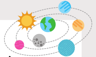
SOLAR SYSTEM
